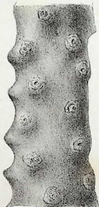
38. Halonia tuberculata .
