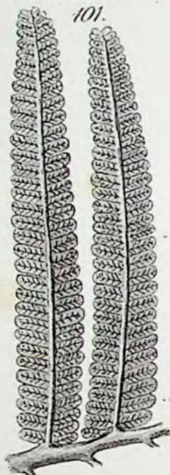
P. parborescens.
