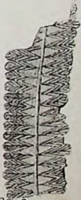
108. Goniopteris elegans.
